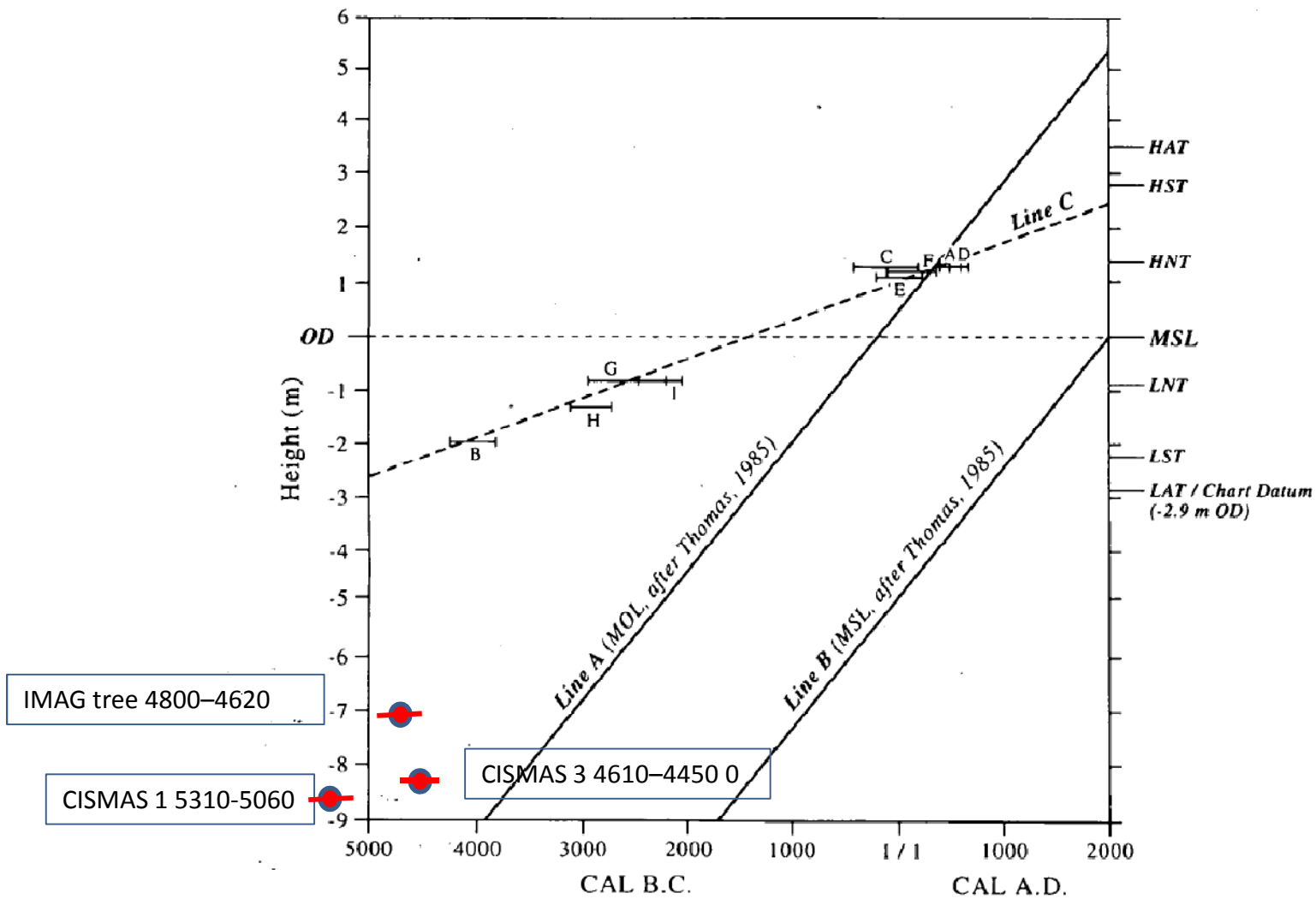
Figure 36 Sea level change in Scilly - Lines A and B after Thomas 1985, Fig 2; Line C, based on calibrated date ranges for selected intertidal 'peat' samples - A = Par Beach (GU-5062), B = Par Beach (GU-5061), C = Crab's Ledge (GU-5059), D = Crab's Ledge (GU-5058), E = Crab's Ledge (GU-5057), F = Crab's Ledge (GU-5056), G = Porth Mellon (GU-5396), H = Porth Mellon (GU-5394), I = Porth Mellon (GU-5392).
